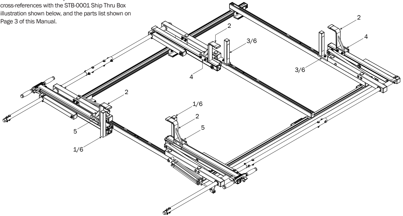
STB-0001 Ship Thru Box
